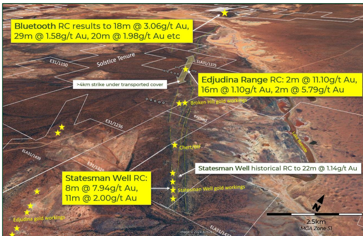
Figure 6: Oblique view looking NW showing the Bluetooth, Edjudina Range 3 and Statesman Well 4 Prospects aligned along the same litho-structural trend.
