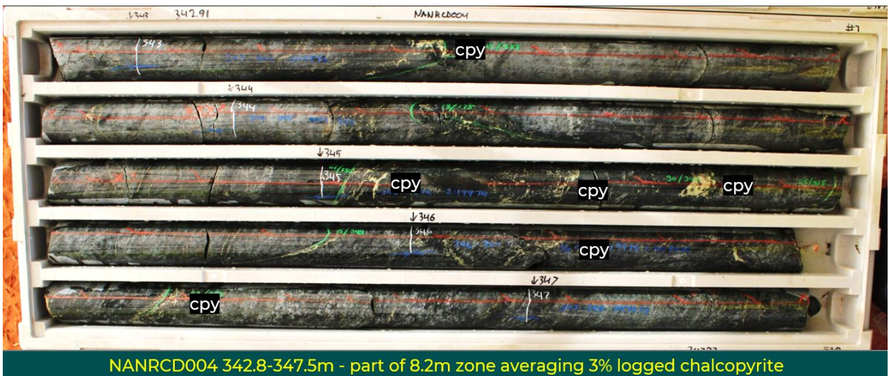
Photo 1. Core tray photo of altered and foliated gabbro 342.8m to 347.5m (4.7m), with chalcopyrite (cpy) sulphide zones labelled. This tray is part of an 8.2m zone averaging 3% logged visual chalcopyrite* (Table 1).
