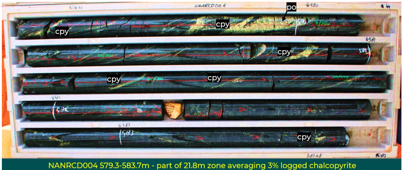
NANRCD004 579.3-583.7m - part of 21.8m zone averaging 3% logged chalcopyrite Photo 4. Core tray photos of foliated mafic from 579.3m to 583.7m (4.4m), with chalcopyrite (cpy) and pyrrhotite (po) sulphide zones labelled. This tray is part of a 21.8m zone averaging 3% logged visual* chalcopyrite (Table 1).
